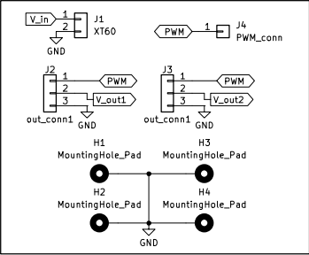
Connectors/Mounting
