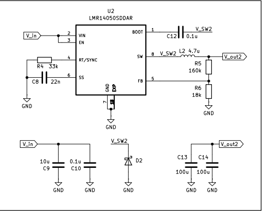
Regulator 2
