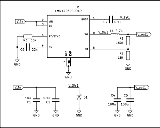
Regulator 1
