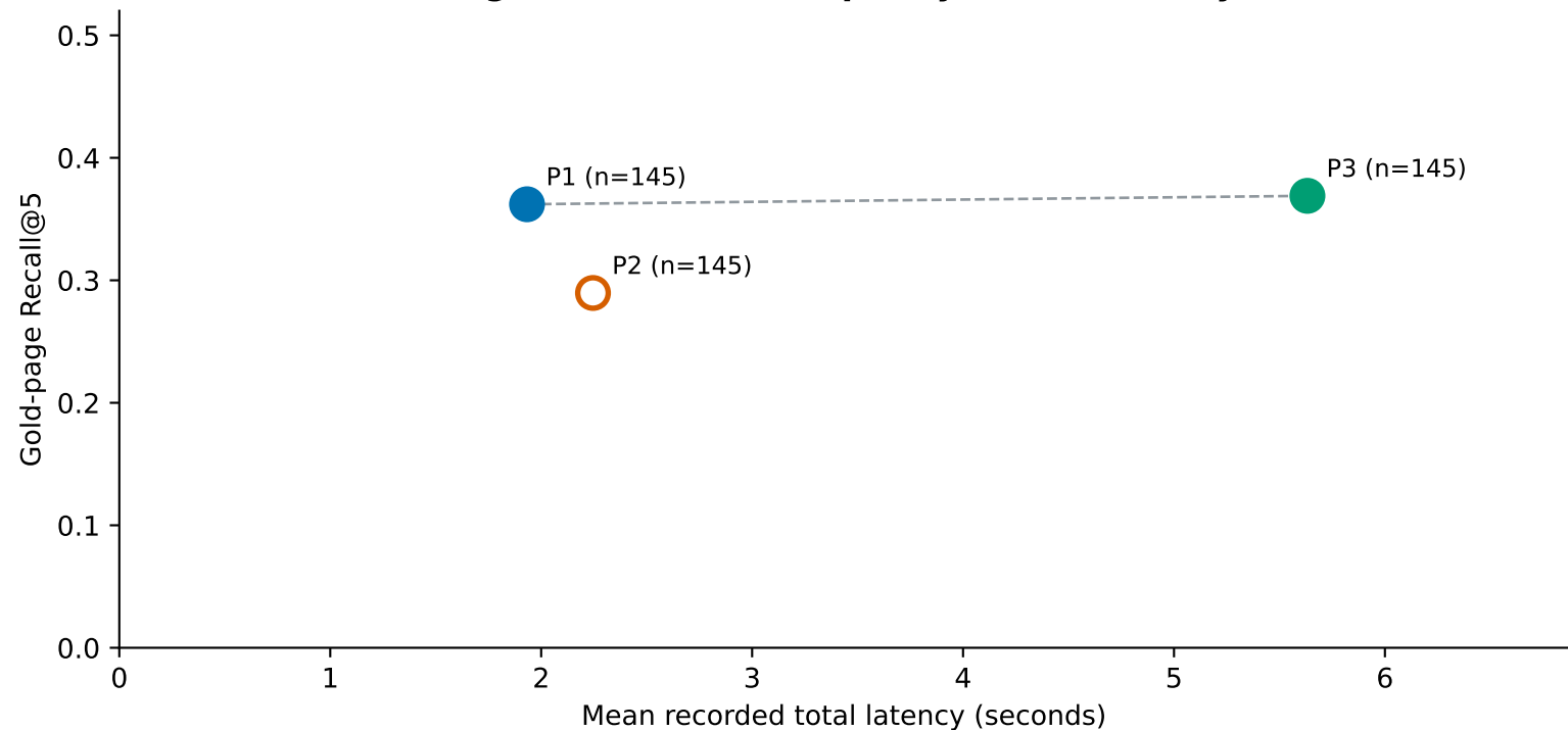
Figure 6b. Retrieval quality versus latency
