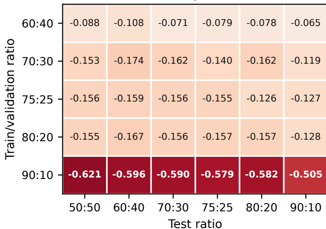
(c) Paired flip 20%: \Delta MCC
