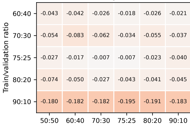
(c) Paired flip 20%: \Delta MCC
