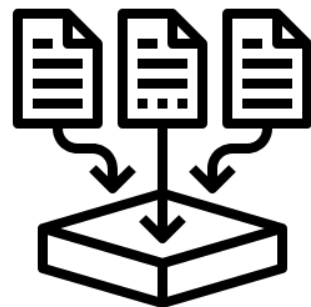
Merging data
