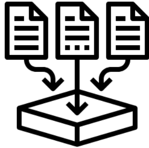
Merging data
