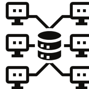
Database handling
