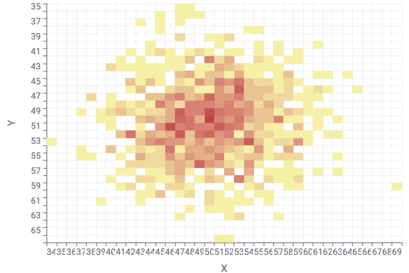
Heatmap
