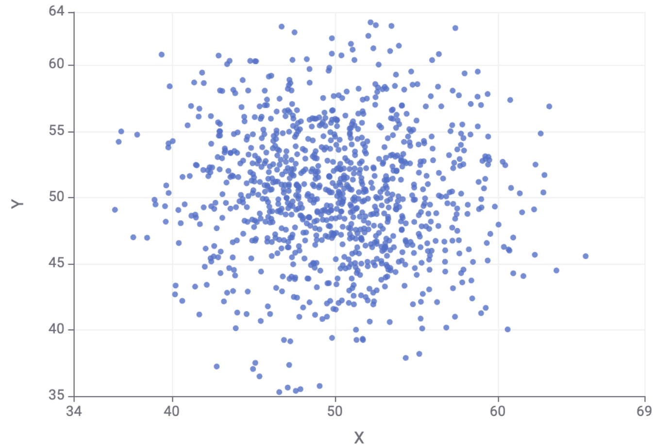
Scatter Plot
