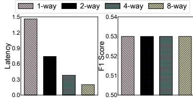
Figure 12: Evaluation of Parallel Execution.
