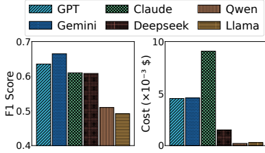
Figure 18: Ablation Study of Different LLMs.
