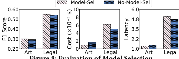
Figure 8: Evaluation of Model Selection.
