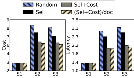
Figure 5: Evaluation of Filter Reordering.
