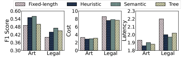
Figure 16: Ablation Study of Chunking Strategies.
