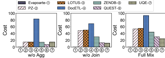
Figure 14: Average Cost of Mixed Queries.
