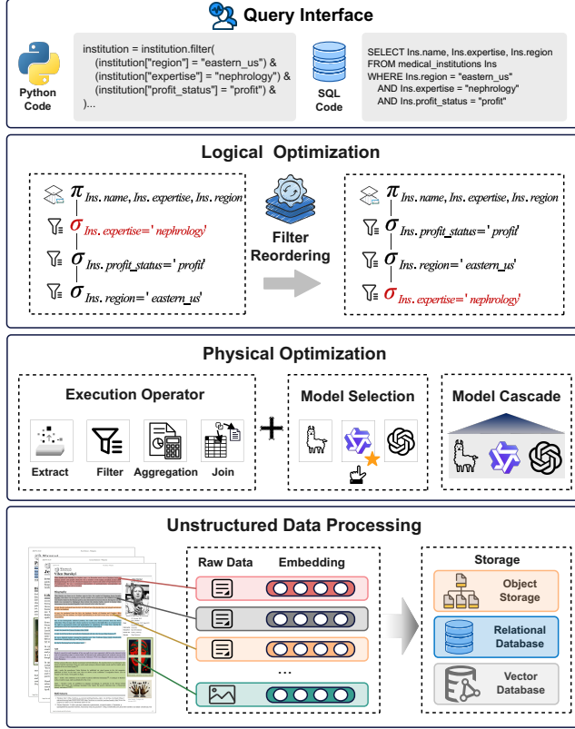
Figure 1: Architecture of Unstructured Data Analysis System.
