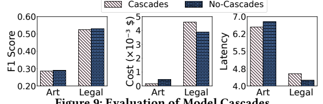
Figure 9: Evaluation of Model Cascades.
