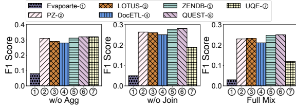
Figure 13: Average F1-score of Mixed Queries.
