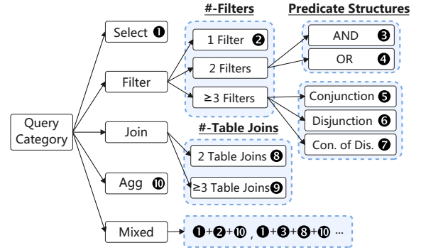
Figure 2: Query Categories.
