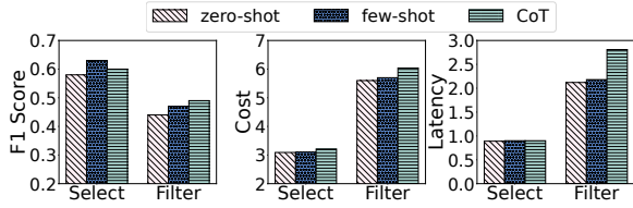
Figure 17: Ablation Study of Prompts.
