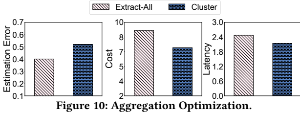
Figure 10: Aggregation Optimization.
