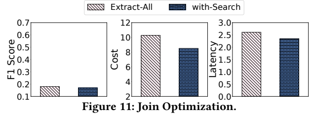
Figure 11: Join Optimization.
