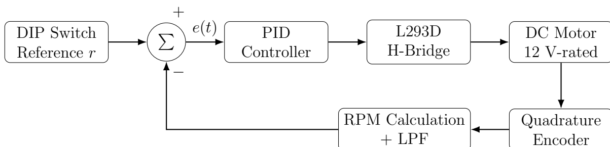
Figure 1: Closed-loop DC motor speed-control block diagram.
