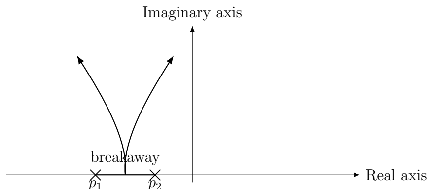
Figure 2: Qualitative root-locus sketch of a second-order DC motor model.
