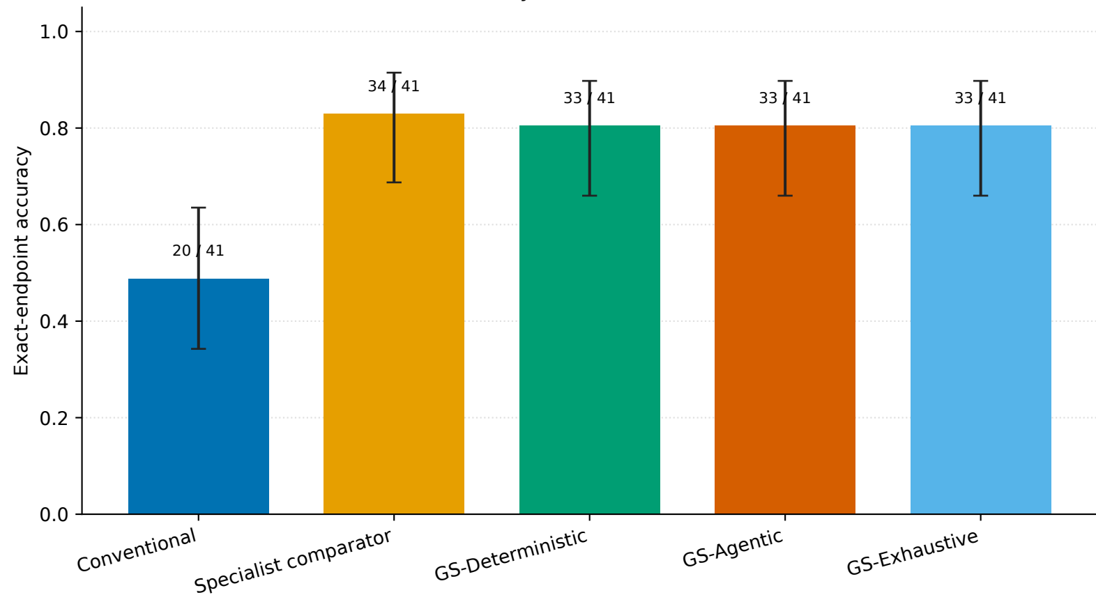
M60 overall accuracy (N = 41 truth-evaluable cases)
