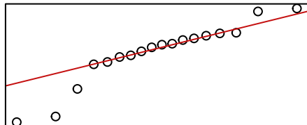
Q-Q Plot of datos$fat
