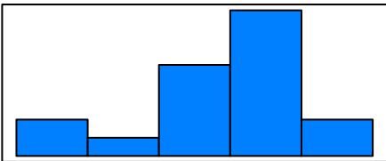
Histogram of datos$fat
