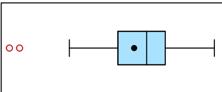
Boxplot of datos$fat
