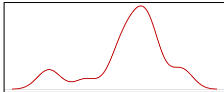
Density of datos$fat
