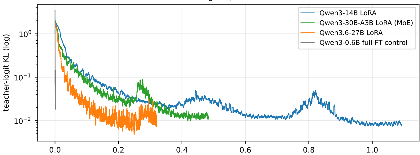
Training KL (smoothed)
