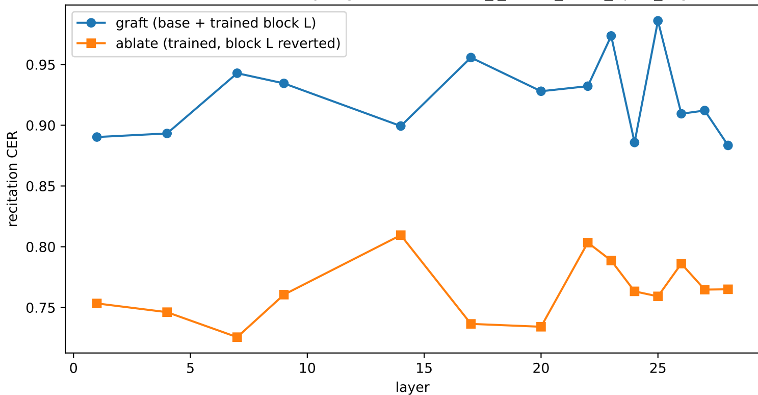
Causal localization: layer graft/ablate — lw_i_vocab_strict_0p6b_rag
