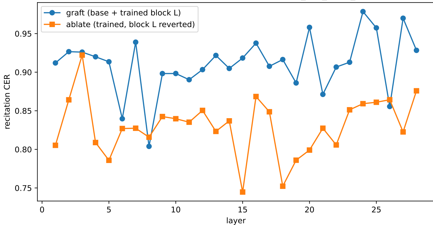
Causal localization: layer graft/ablate — lw_seq_0p6b_rag
