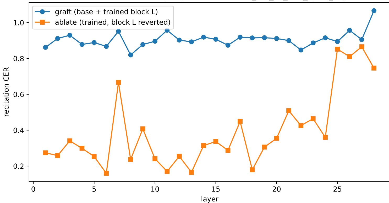
Causal localization: layer graft/ablate — lw_tail_ce_e40_0p6b_rag
