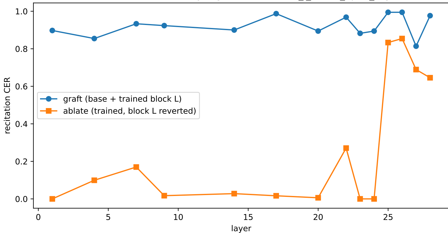
Causal localization: layer graft/ablate — lw_i_l2mse_0p6b_rag
