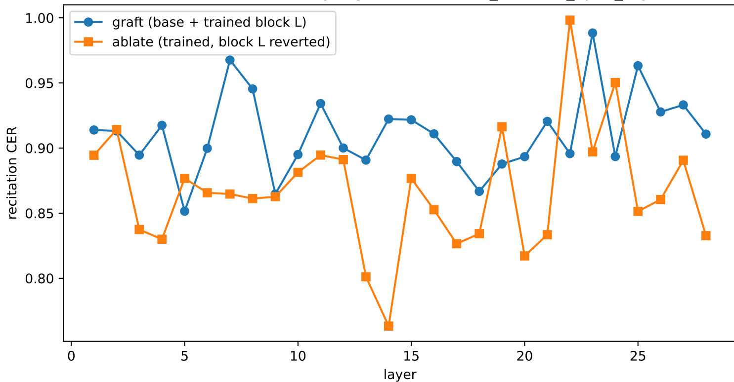
Causal localization: layer graft/ablate — lw_summed_0p6b_rag
