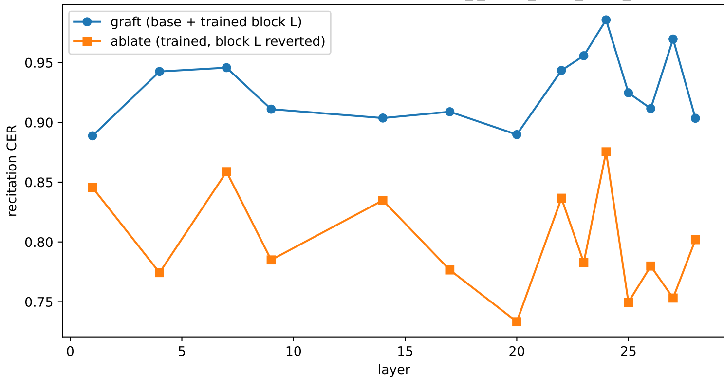
Causal localization: layer graft/ablate — lw_i_nmse_strict_0p6b_rag
