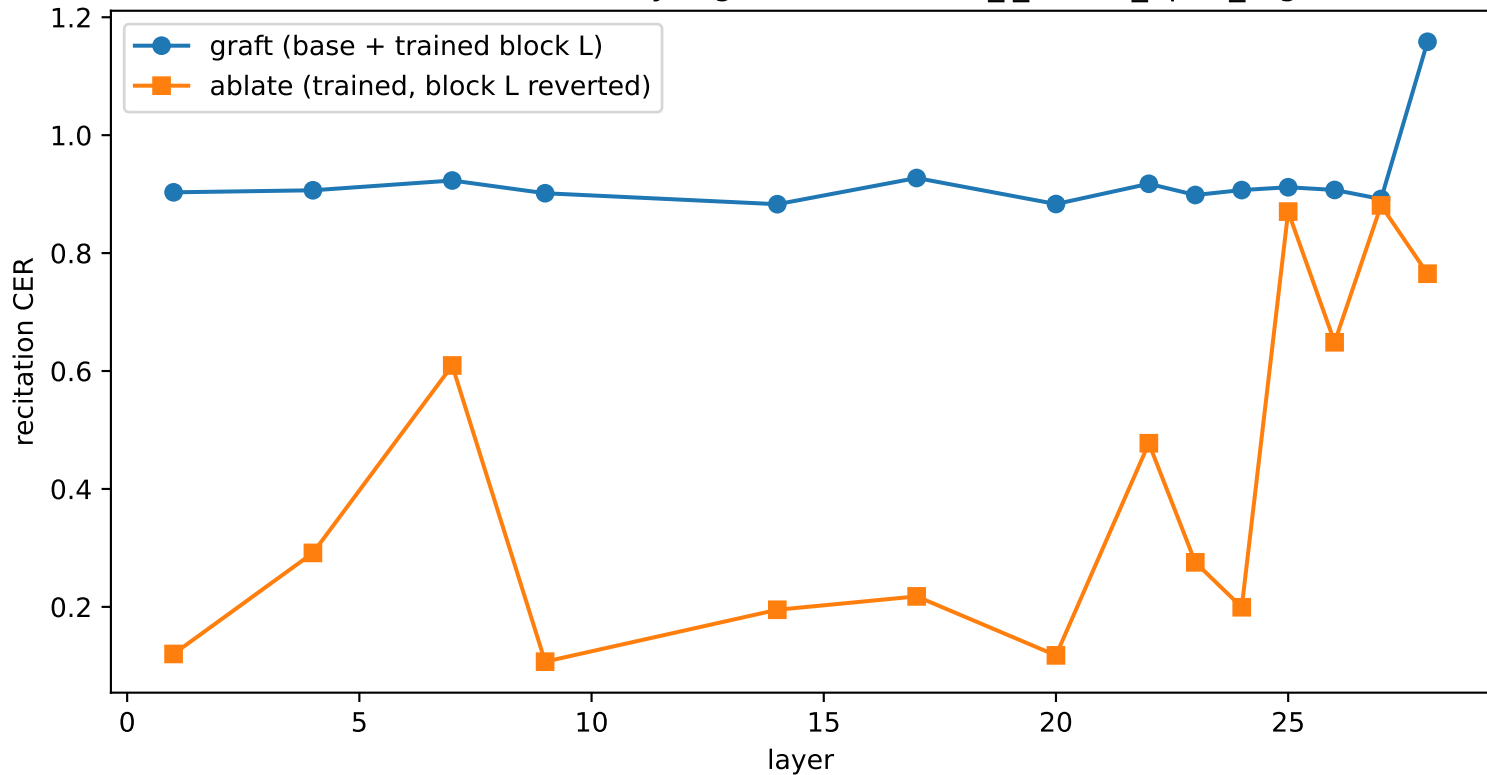
Causal localization: layer graft/ablate — lw_i_cosine_0p6b_rag
