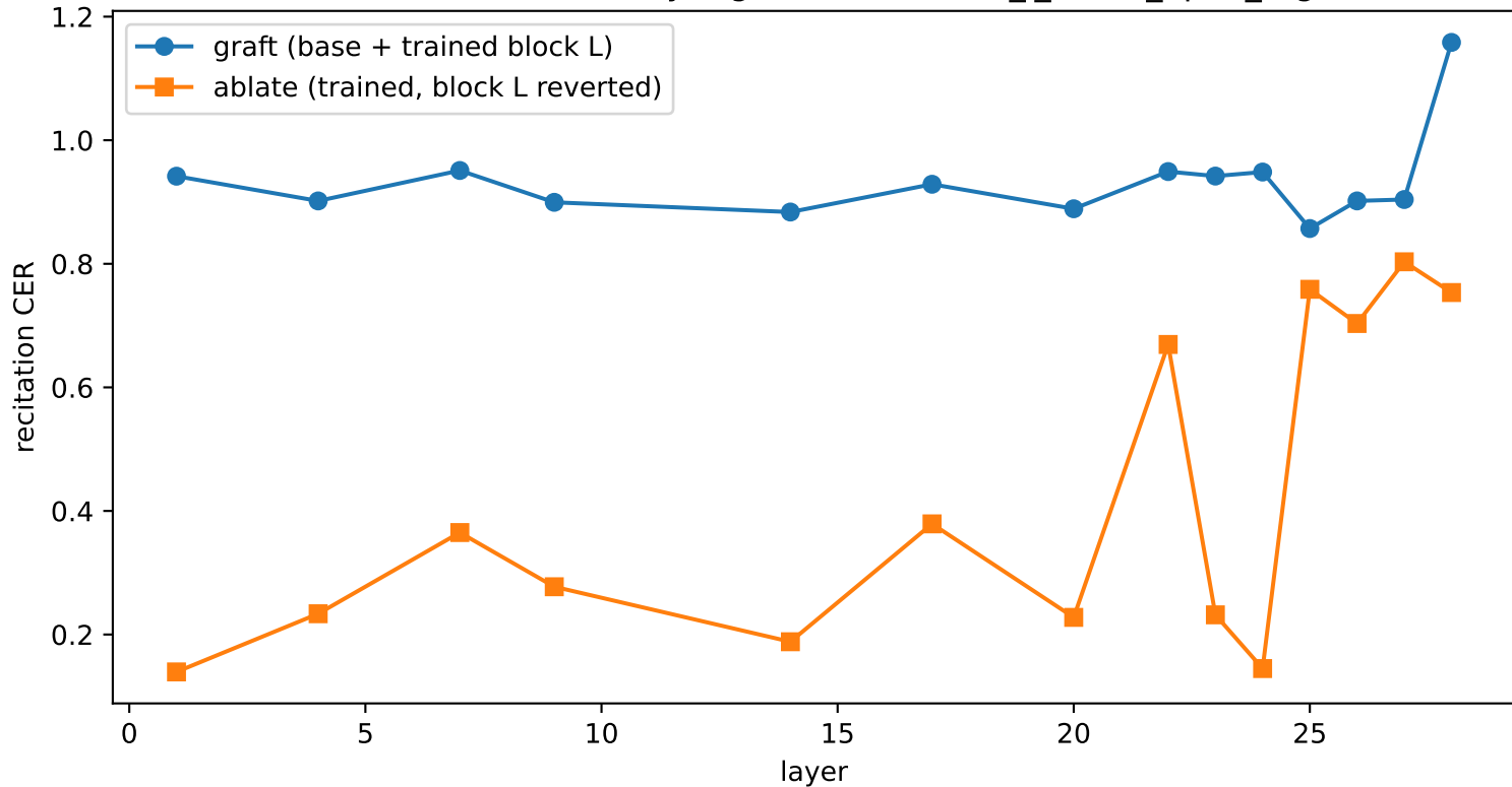
Causal localization: layer graft/ablate — lw_i_huber_0p6b_rag
