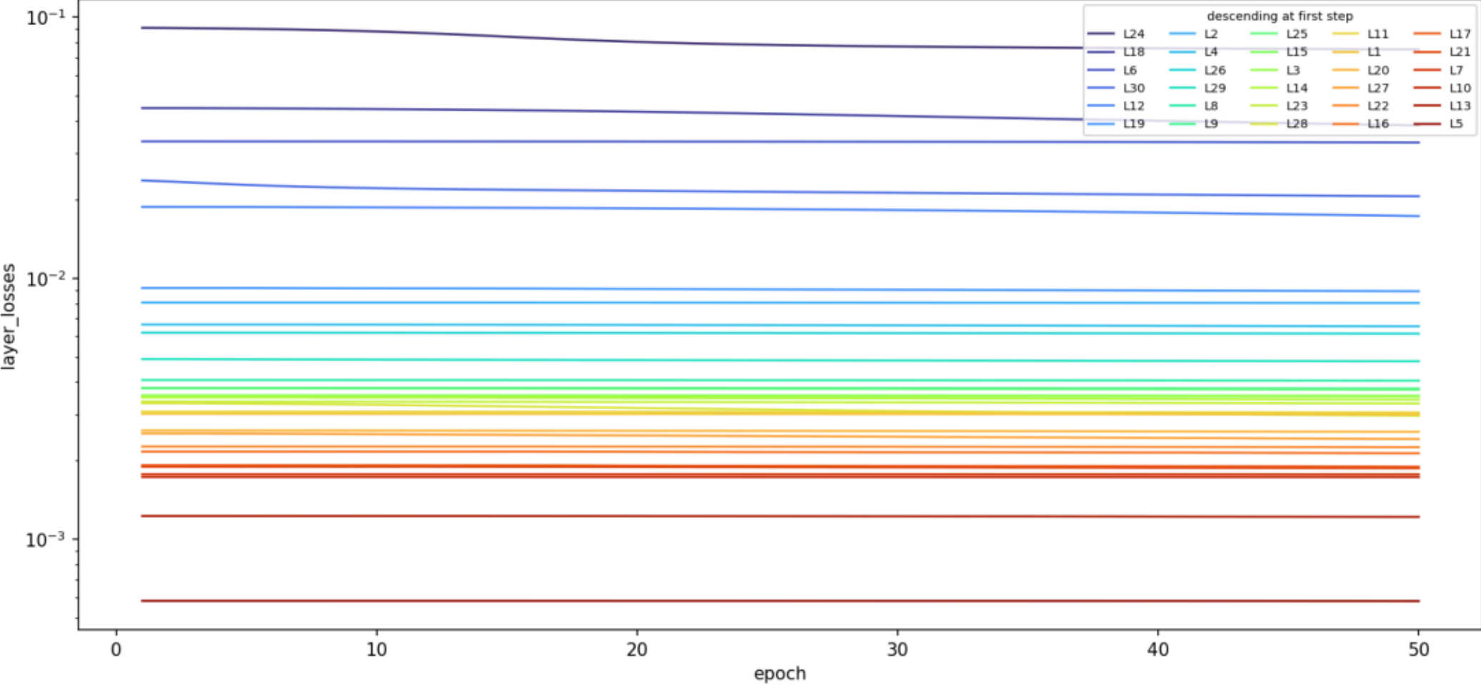
Block-local loss by epoch and layer
