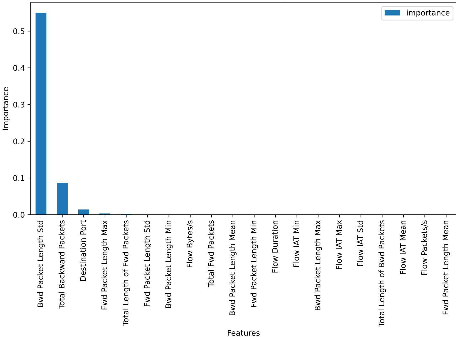
DDoS1 Attack - Feature Importance
