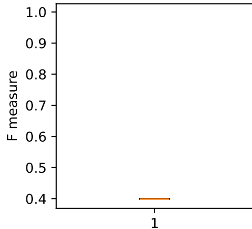
PortScan - AdaBoost
