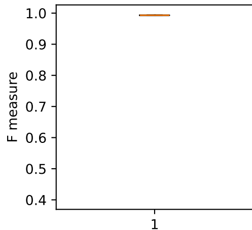
PortScan - AdaBoost
