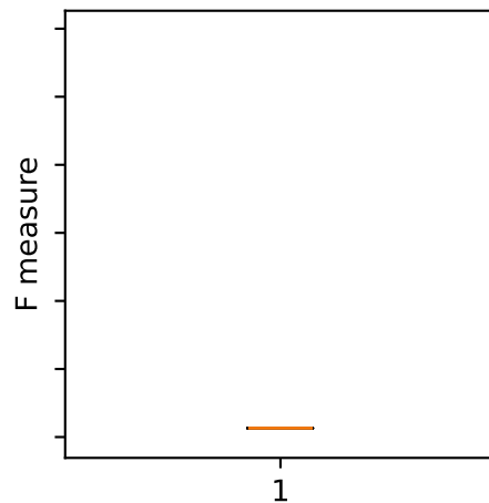
PortScan - MLP
