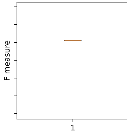
PortScan - MLP
