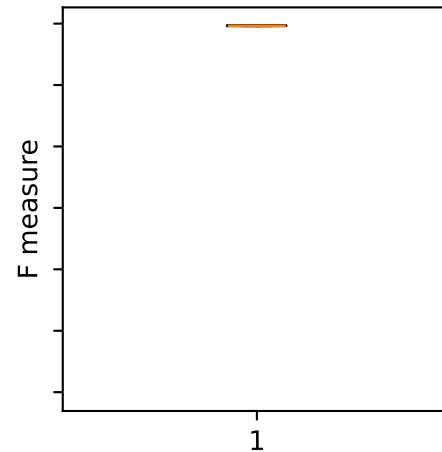
PortScan - ID3
