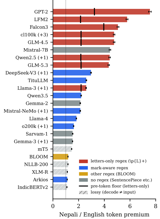
Figure 2: Nepali/English premium of 24 distinct tokenizers (33 released; “+ n ” counts aliases) on FLORES-200 devtest, with 95% paired-bootstrap intervals. Black ticks mark the pre-token floor of each letters-only tokenizer: no merge-based extension can move its bar to the left of the tick. Dotted line: parity with English.
