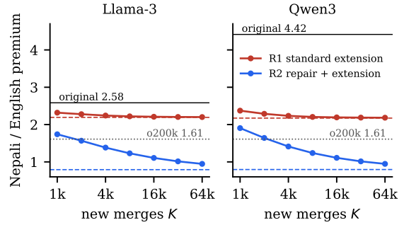
Figure 3: Nepali/English premium on FLORES-200 devtest after adding K merges by continued BPE, under the letters-only regex (R1) and the repaired regex (R2). Dashed lines: pre-token floors under each model’s own pattern (2.19 and 2.17 letters-only; 0.79 and 0.80 repaired, for Llama-3 and Qwen3). 95% paired-bootstrap intervals (half-width at most 0.03) are narrower than the markers.
