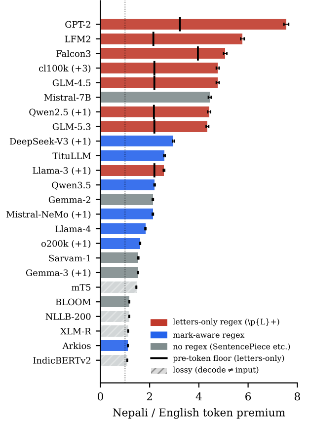
Fig. 2. Nepali/English premium of 24 distinct tokenizers (33 released; “+n” counts aliases) on FLORES-200 devtest, with 95% paired-bootstrap intervals. Black ticks mark the pre-token floor of each letters-only tokenizer: no merge-based extension can move its bar to the left of the tick.
