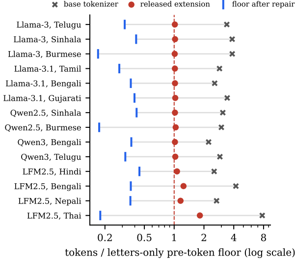
Fig. 1. Released merge-based extensions of letters-only models on FLORES-200 devtest of each target language, relative to the letters-only pre-token floor. The ten extensions by Yamaguchi et al. (top) move from the base tokenizer ( \times ) to within 4% of the floor ( \bullet ). LFM2.5 (bottom) stops further above it for Bengali and Thai. The blue tick is the floor under the repaired regex. Full numbers, including the Amharic control, are in Table VI.
