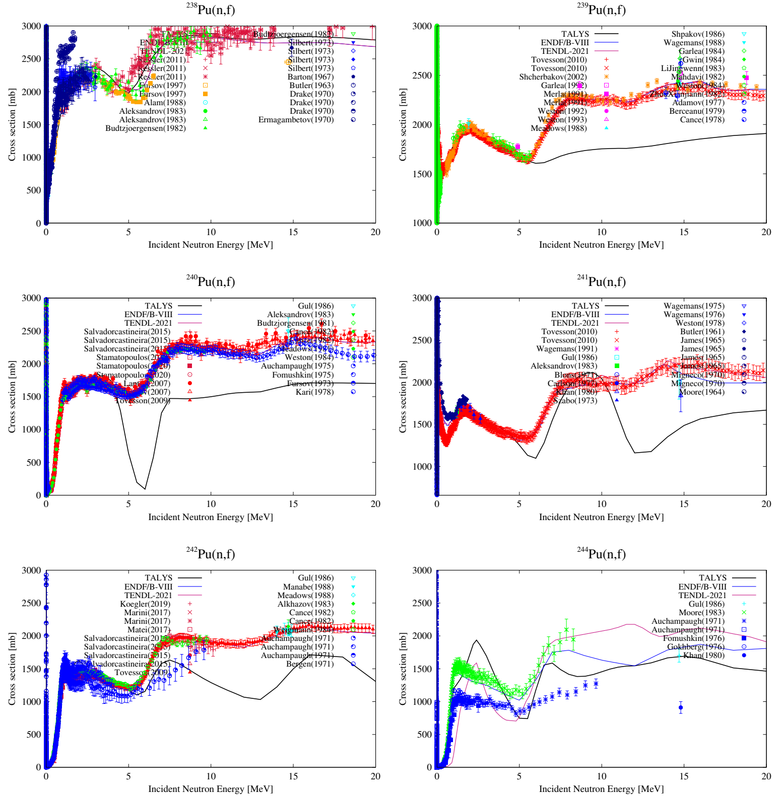
Figure 6.8: Fission cross sections for Pu isotopes.
