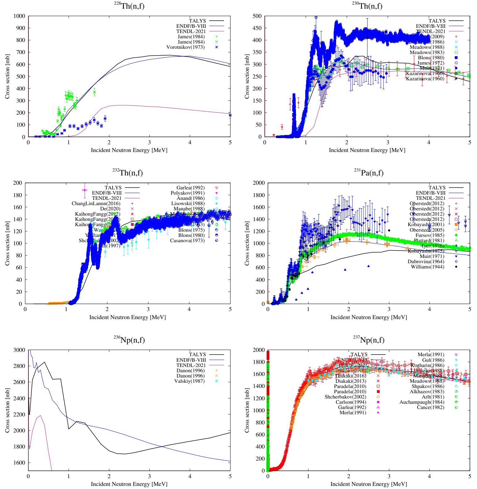
Figure 6.1: Fission cross sections for Th, Pa and Np isotopes.
