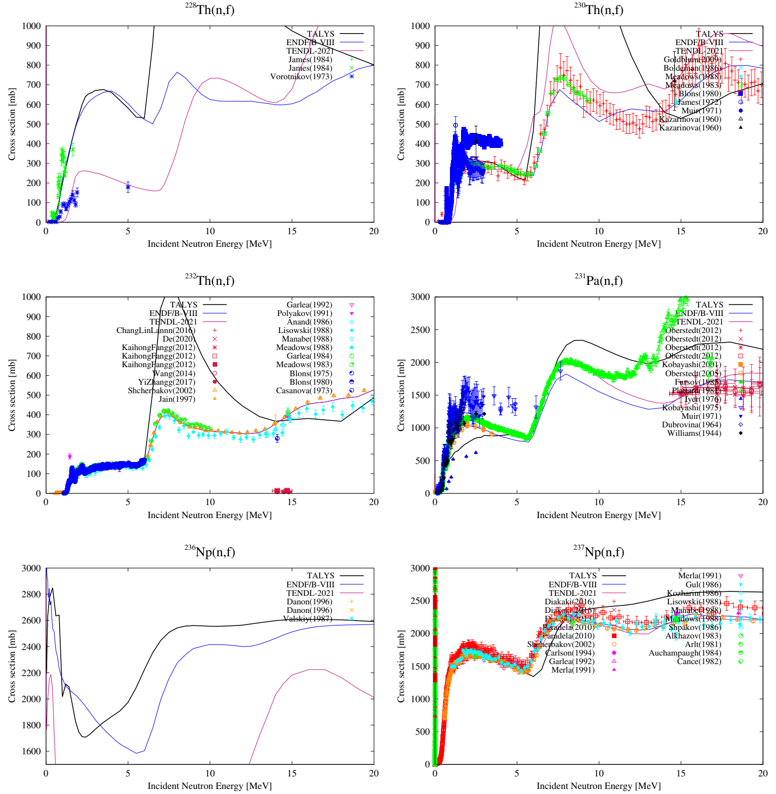
Figure 6.6: Fission cross sections for Th, Pa and Np isotopes.
