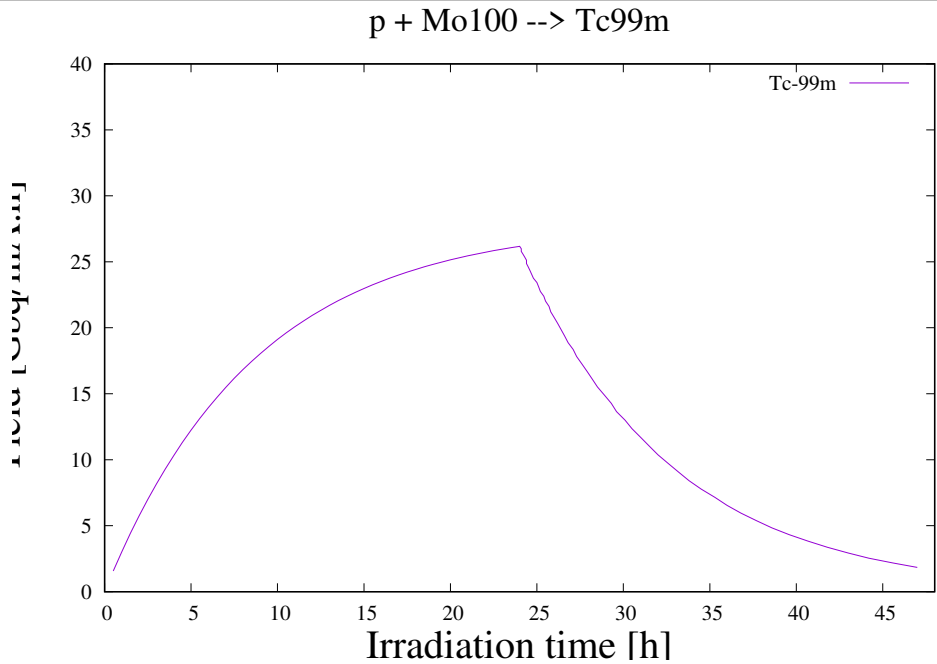
Figure 7.1: Production of Tc-99m
