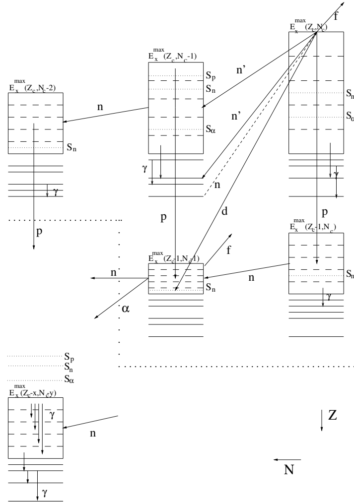
Figure 5.3: Neutron-induced reaction. The dashed arrow represents the incident channel, while the continuous arrows represent the decay possibilities. E_x^{max} denotes the maximal possible excitation energy of each nucleus and S_k is the particle separation energy for particle k . For each nucleus a few discrete levels are drawn, together with a few continuum energy bins. Spin and parity degrees of freedom are left out of this figure for simplicity. Fission is indicated by an f .
