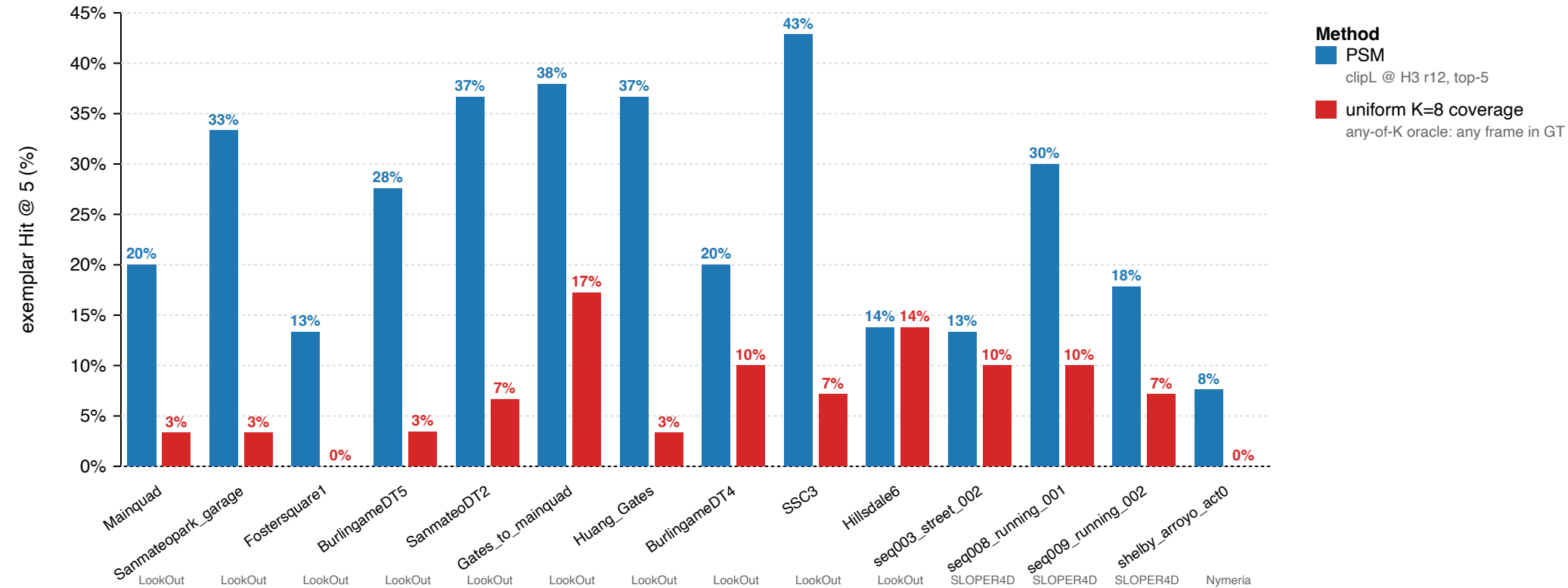
PSM vs any-of-K coverage (K=8 uniform frames)
