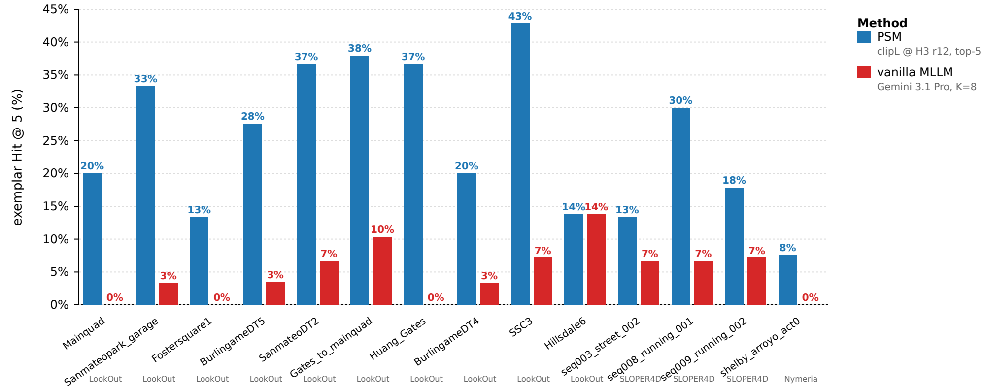
PSM vs vanilla MLLM (Hit @ 5, K=8 candidates)
