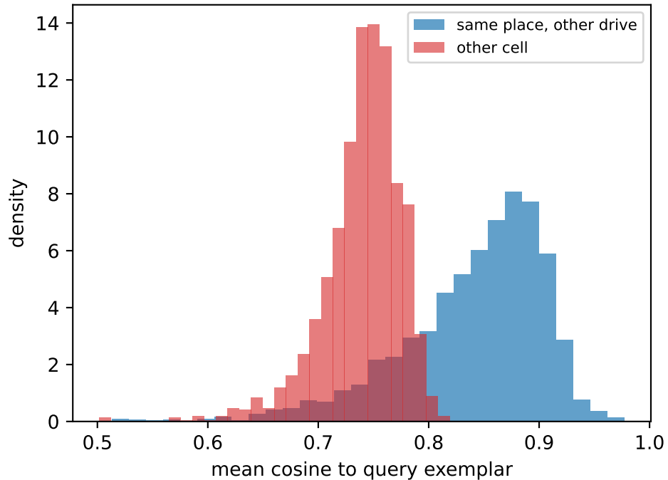
Cross-session place similarity
