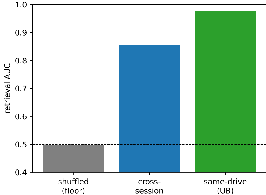
Cross-session retrieval AUC
