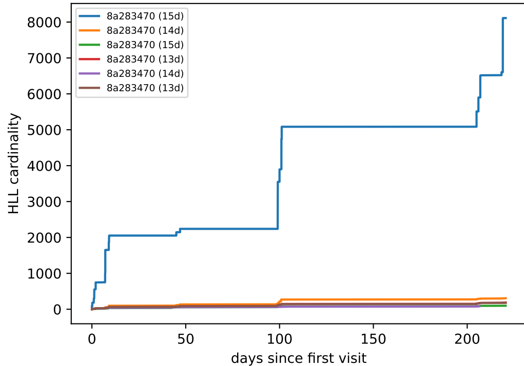
Accrual across drives (bounded 1024 B/cell)
