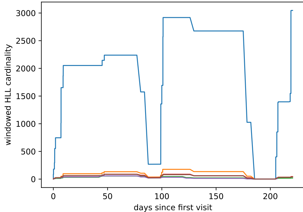
Ring-buffer time-decay (windowed)
