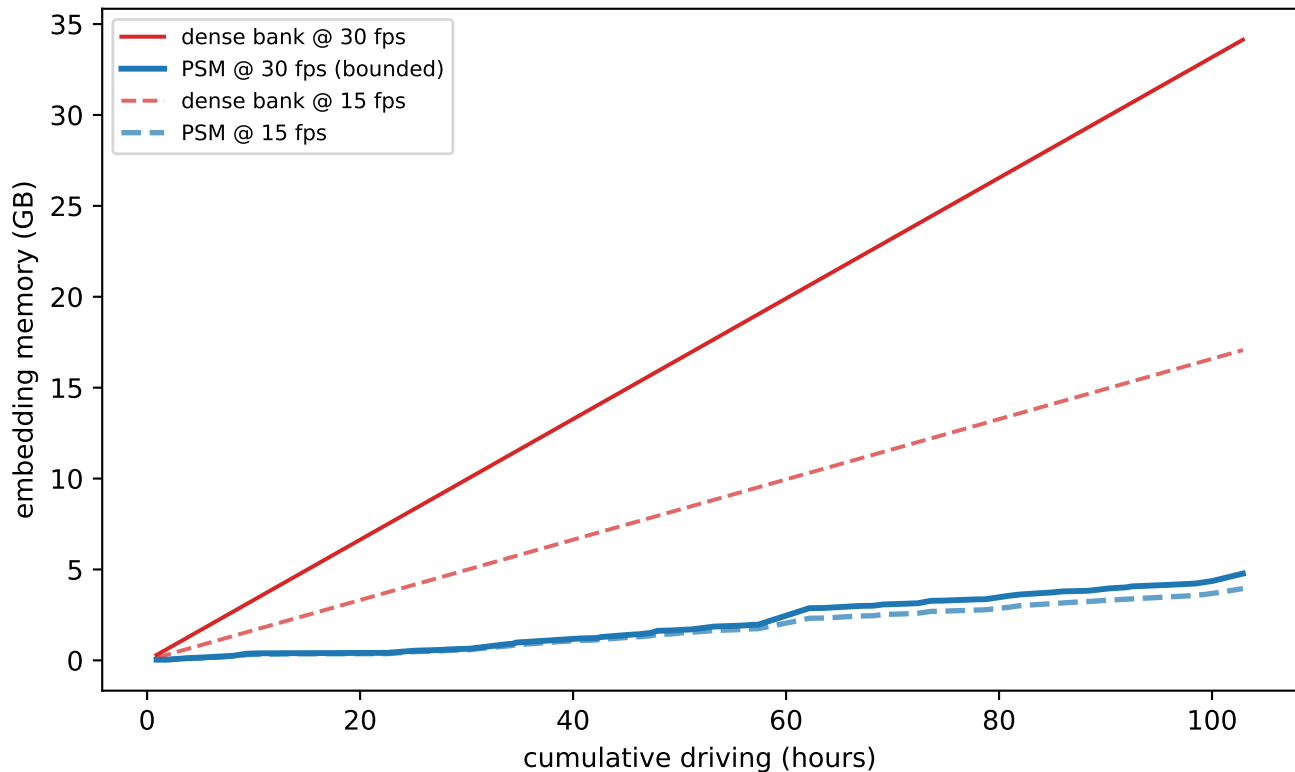
HDD: PSM area-bounded reservoir vs. dense embedding bank
