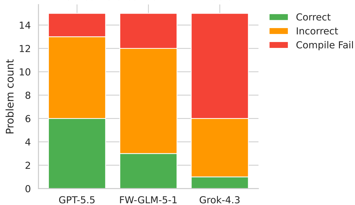
Outcome breakdown — All Tools
