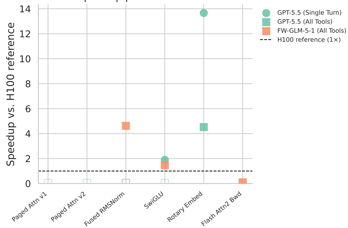
Speedup per solved kernel
