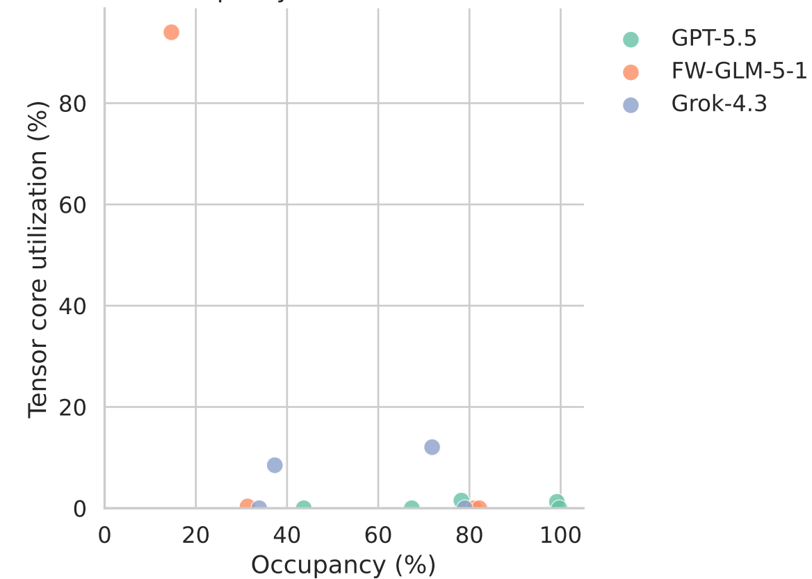
Occupancy vs. tensor core use
