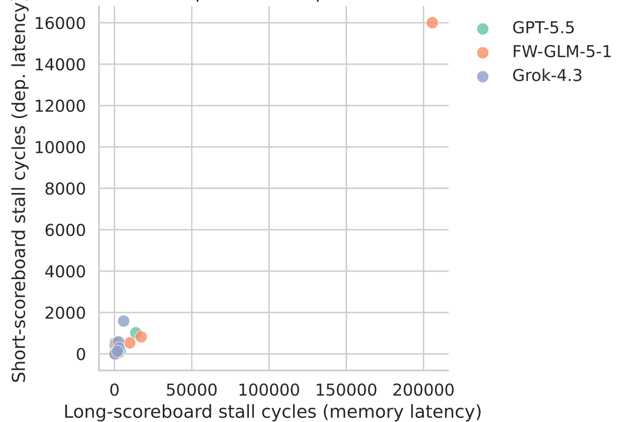
Warp stall decomposition
