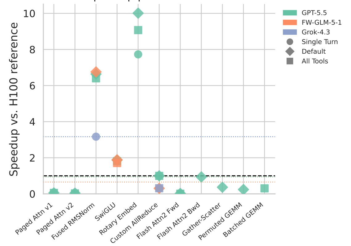
Speedup per solved kernel
