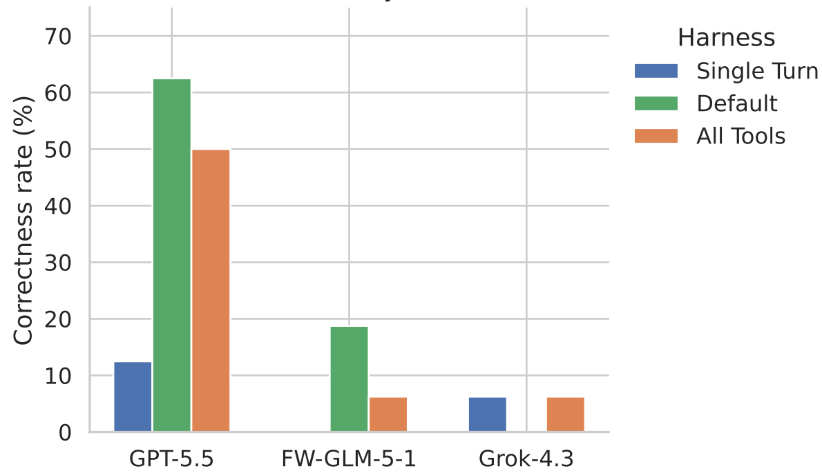
Outcome breakdown by harness
