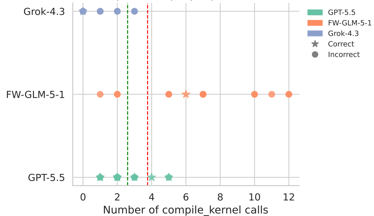
Compile attempts per problem (AT)
