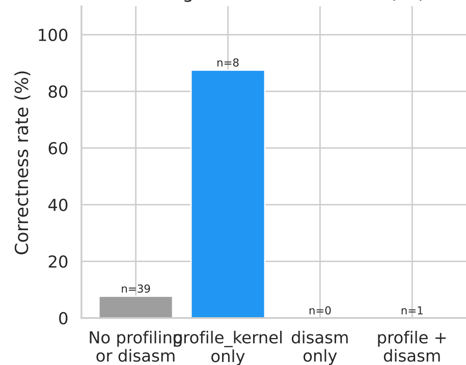
Profiling tools vs. correctness (AT)
