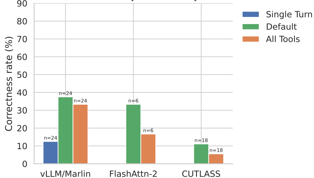
Correctness by kernel family
