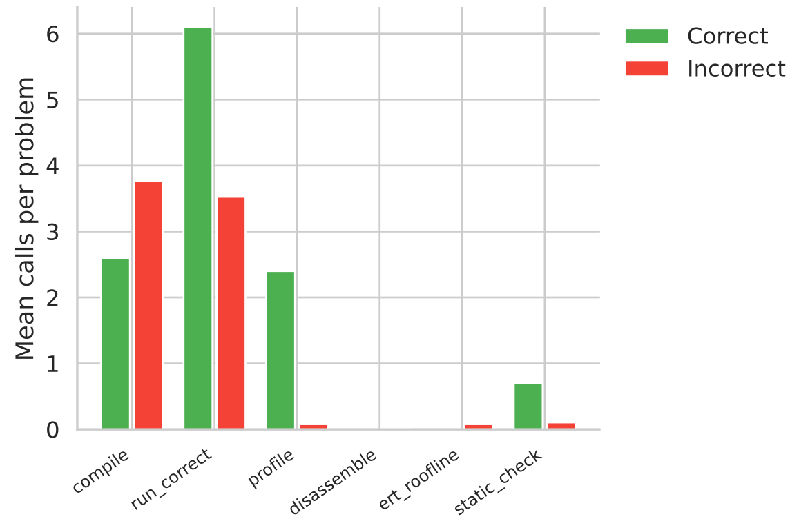
Tool calls: correct vs. incorrect (AT)
