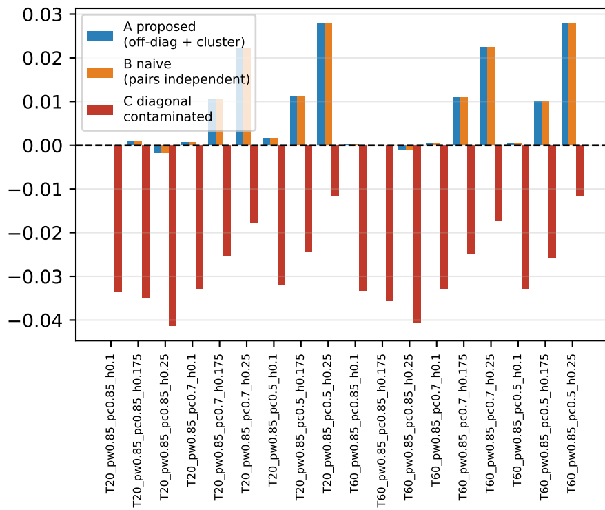
Bias of \hat{\Delta}
