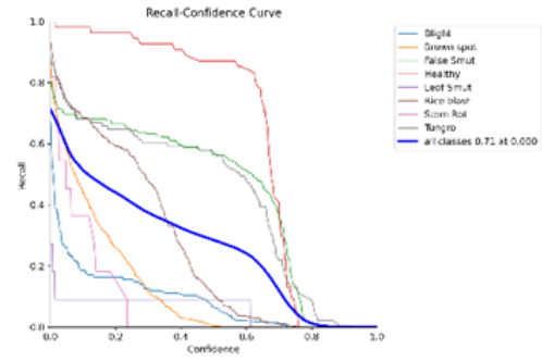
Fig. 10. Recall Curve (R Curve)
