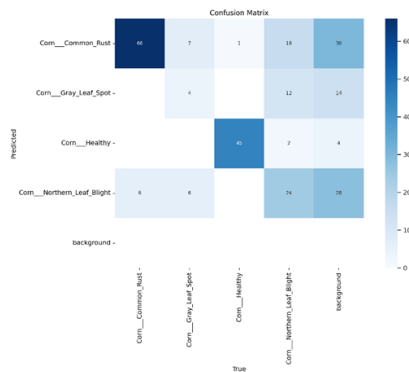
Fig. 3. Confusion Matrix for Maize Disease Detection
