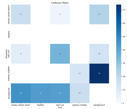
Fig. 2. Confusion Matrix for Wheat Disease Detection
