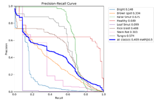
Fig. 11. PR Curve (Precision-Recall Curve)
