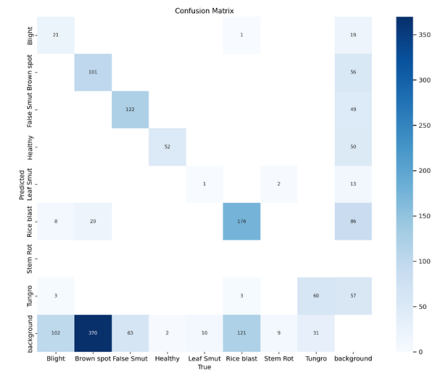
Fig. 1. Confusion Matrix for Rice Disease Detection
