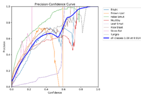
Fig. 9. Precision Curve (P Curve)
