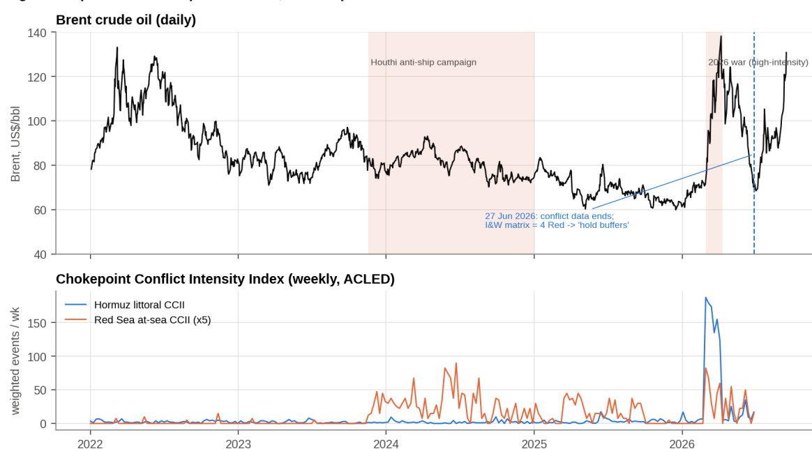
Figure Oil price and chokepoint conflict, 2022-Sep 2026
