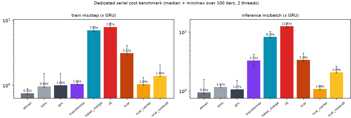
Figure 10: Dedicated serial CPU benchmark. Bars show medians and whiskers show the repeated-iteration minimum and maximum.
