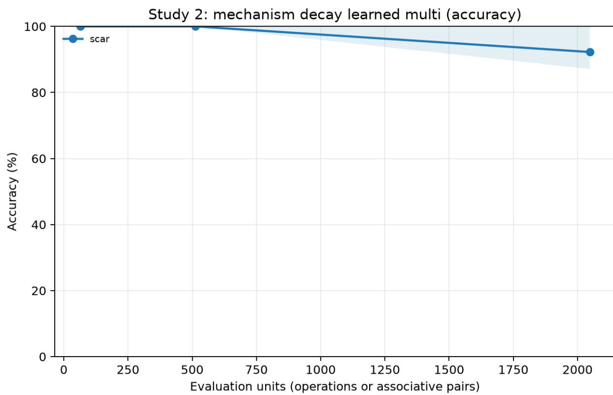
Figure 8: Study 2E: accuracy for the learned multi-timescale decay mechanism variant.
