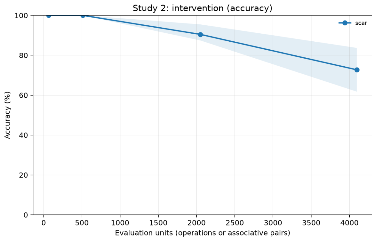
Figure 9: Study 2F: frozen-memory intervention accuracy at the tested evaluation contexts.
