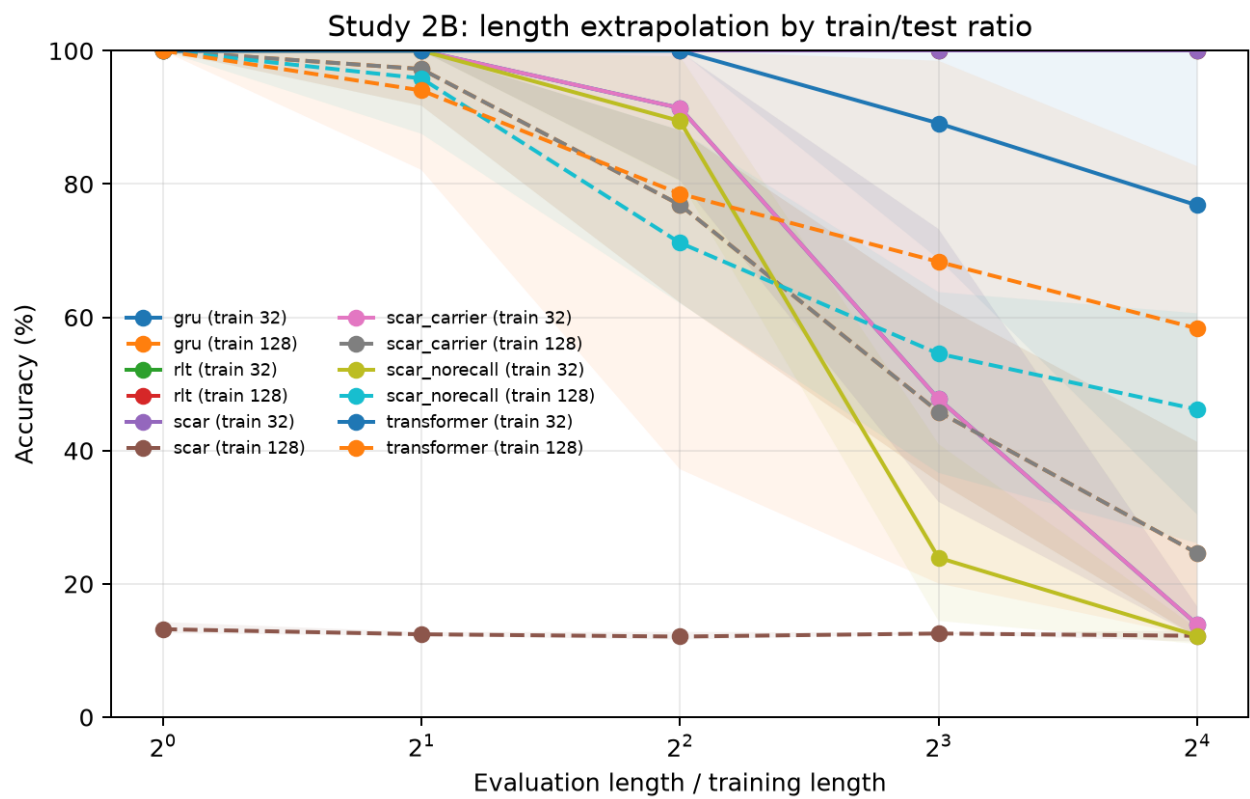
Figure 5: Study 2B: accuracy plotted against evaluation length divided by training length for two training contexts.
