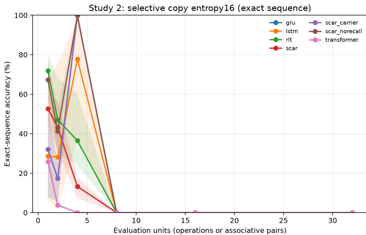
Figure 7: Study 2D: free-running exact-sequence accuracy for high-entropy selective copy.
