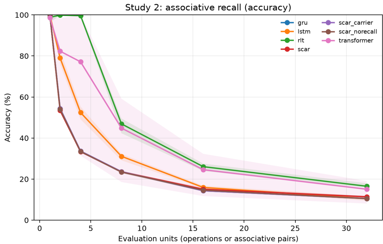
Figure 6: Study 2C: associative key/value recall across the number of presented pairs. Shaded bands are bootstrap intervals over seed means.
