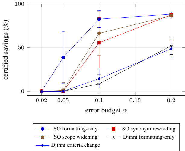
FIGURE 2. The \alpha -savings frontier under the pinned procedure: mean \pm sd over 1,000 sampling replications per point, generated from the result files. Savings collapse as \alpha approaches each column's intrinsic flip rate.
