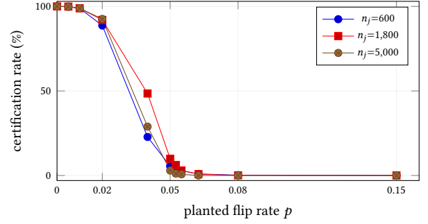
Figure 3: Calibration power at \alpha=0.05 (presented-cells estimand, 2,000 trials per point). Certification rises smoothly as p falls below \alpha and is small but nonzero just above it. There the realized population rate of a planted stratum often falls below \alpha , and certifying it is correct. The unconditional rate of certificates whose realized error exceeds \alpha stays at or below 1.00% in every configuration, against the nominal 5%. The n_j=1,800 curve sits above the other two at intermediate p , because the exact bound’s finite-population correction tightens as the sampled fraction grows. The six-look schedule reaches most of an n_j=1,800 stratum but a minority of an n_j=5,000 one. The n_j=600 stratum’s final look is the whole stratum, which cannot certify, so its deepest certifying look is its fourth.
