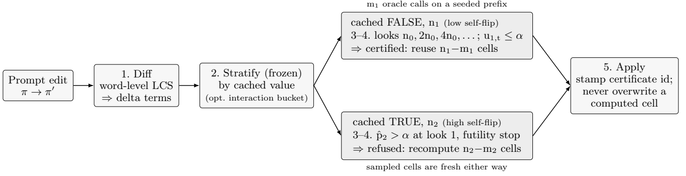
FIGURE 1. The procedure on the configuration our experiments pin. Stratification is frozen before any oracle call, so it moves power but never validity (Assumption 2); only steps 3–4 spend model calls, and they stop on evidence about a stratum’s rate, which is independent of the stratum’s size. The two lanes are the outcome we measure throughout: the stable stratum certifies and is reused under a certificate, while the volatile one is refused at every budget we tried and recomputed. A refusal is a stability diagnosis of that slice of the column (Section II), reached at the cost of one look instead of a full recomputation.
