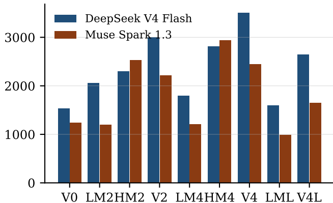
Reasoning tokens per run
