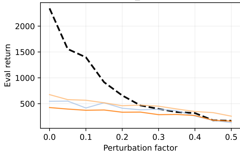
action_replace
