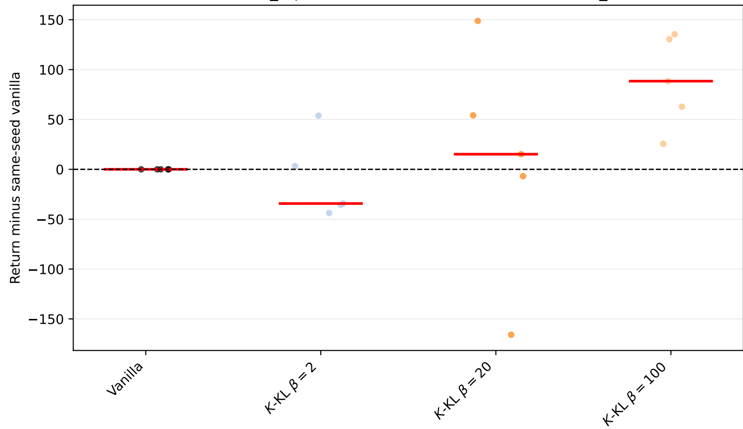
Walker2d-v4 action_replace factor=0.5: seed scatter (vanilla_subtracted)
