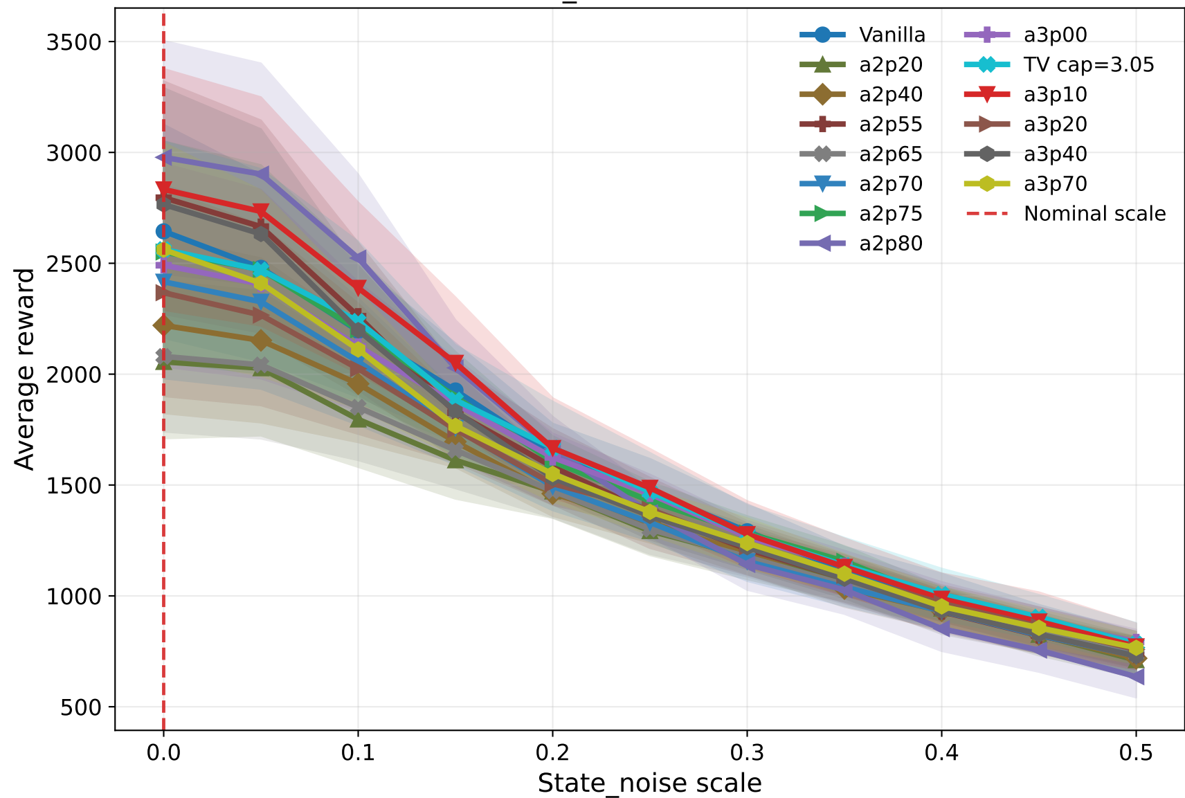
State_noise robustness
