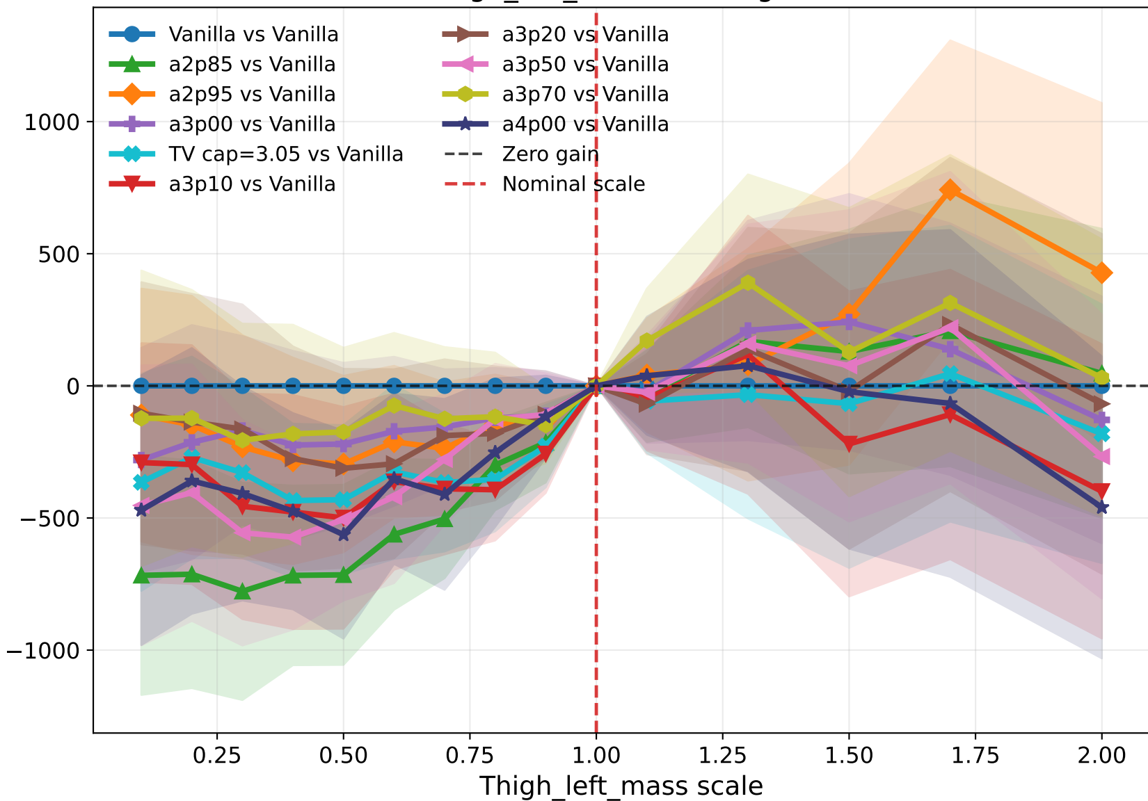
Thigh_left_mass robust gain
