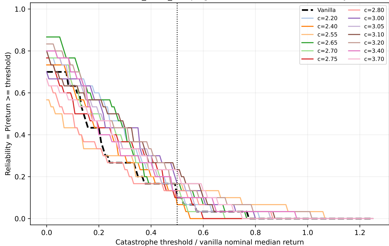
HalfCheetah-v4 friction_mass_damping factor=0.5: robustness reliability curve
