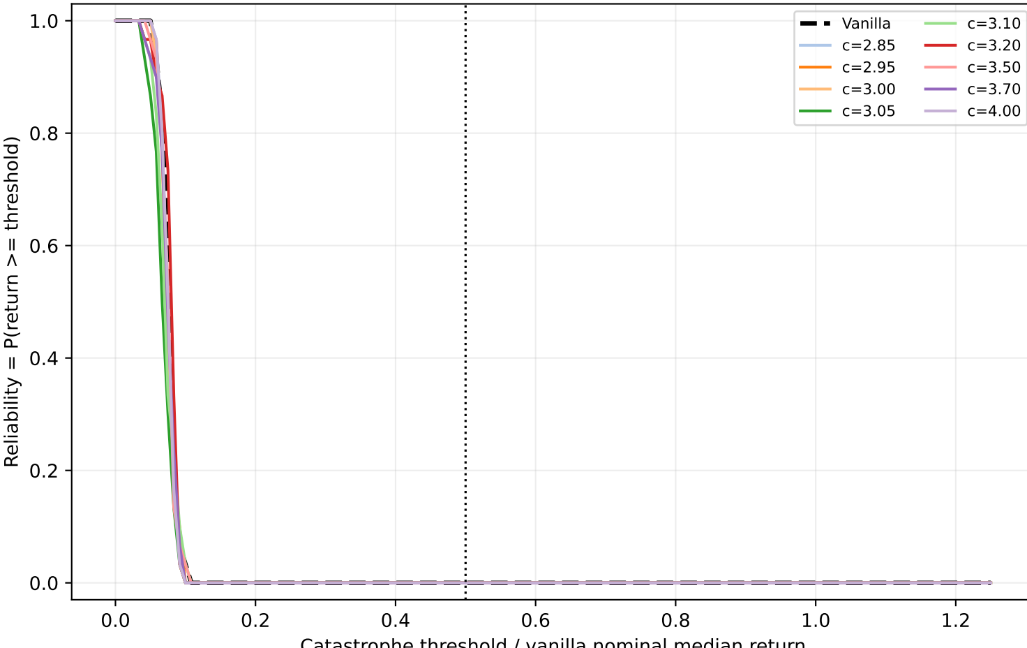
Walker2d-v4 action_replace factor=0.5: robustness reliability curve
