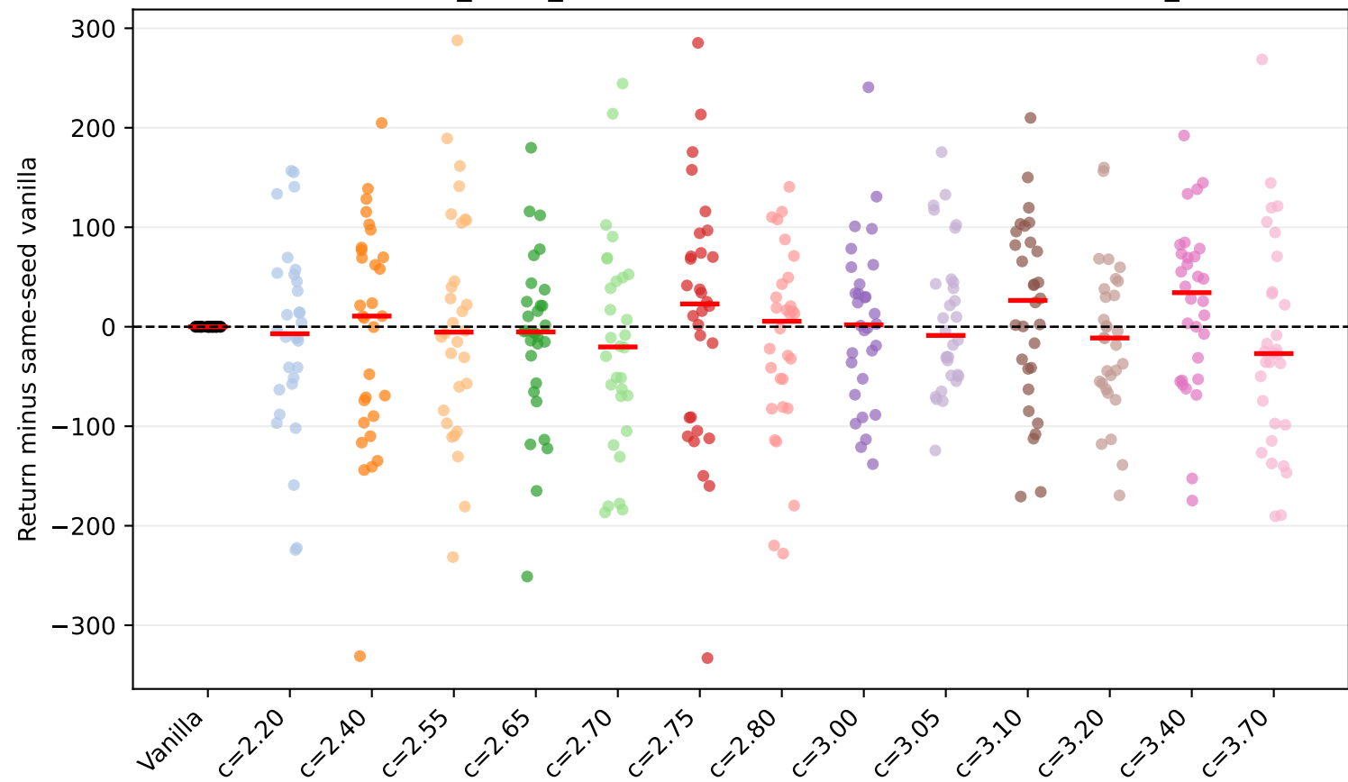
HalfCheetah-v4 action_noise_bernoulli factor=0.5: seed scatter (vanilla_subtracted)
