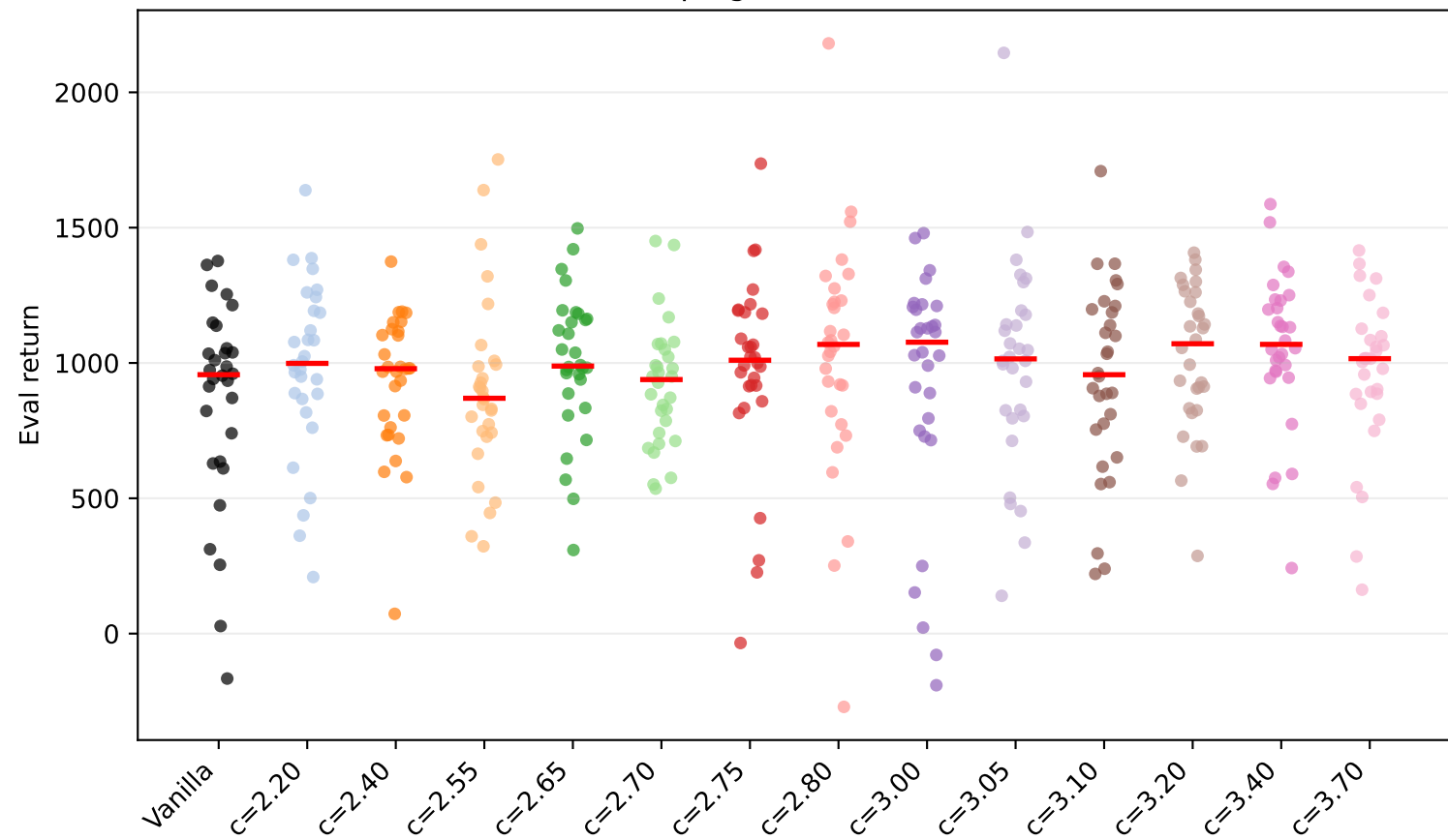
HalfCheetah-v4 damping factor=0.5: seed scatter (raw)
