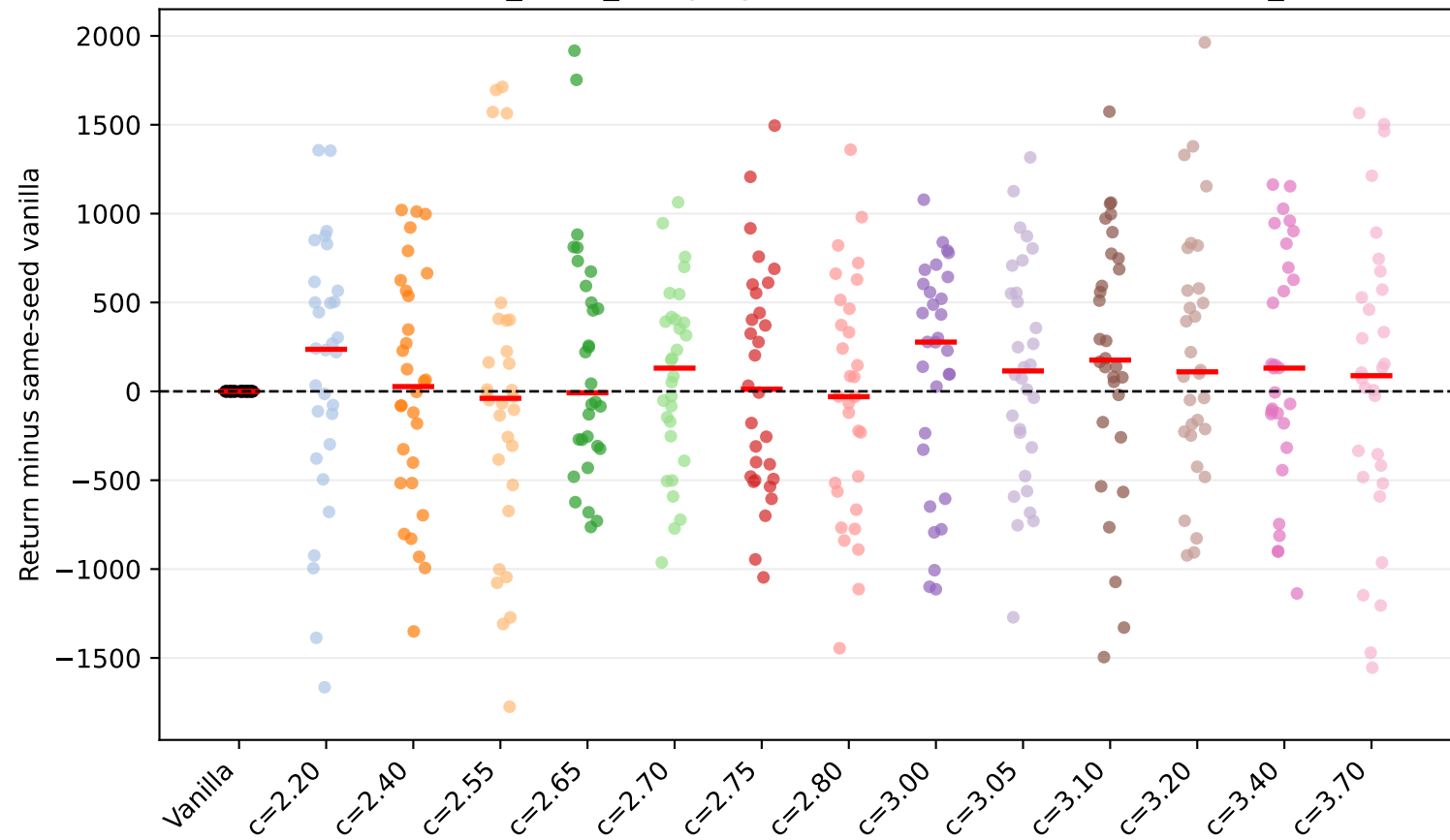
HalfCheetah-v4 friction_mass_damping factor=0.5: seed scatter (vanilla_subtracted)
