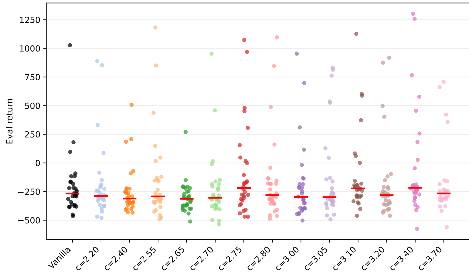
HalfCheetah-v4 gear factor=0.5: seed scatter (raw)
