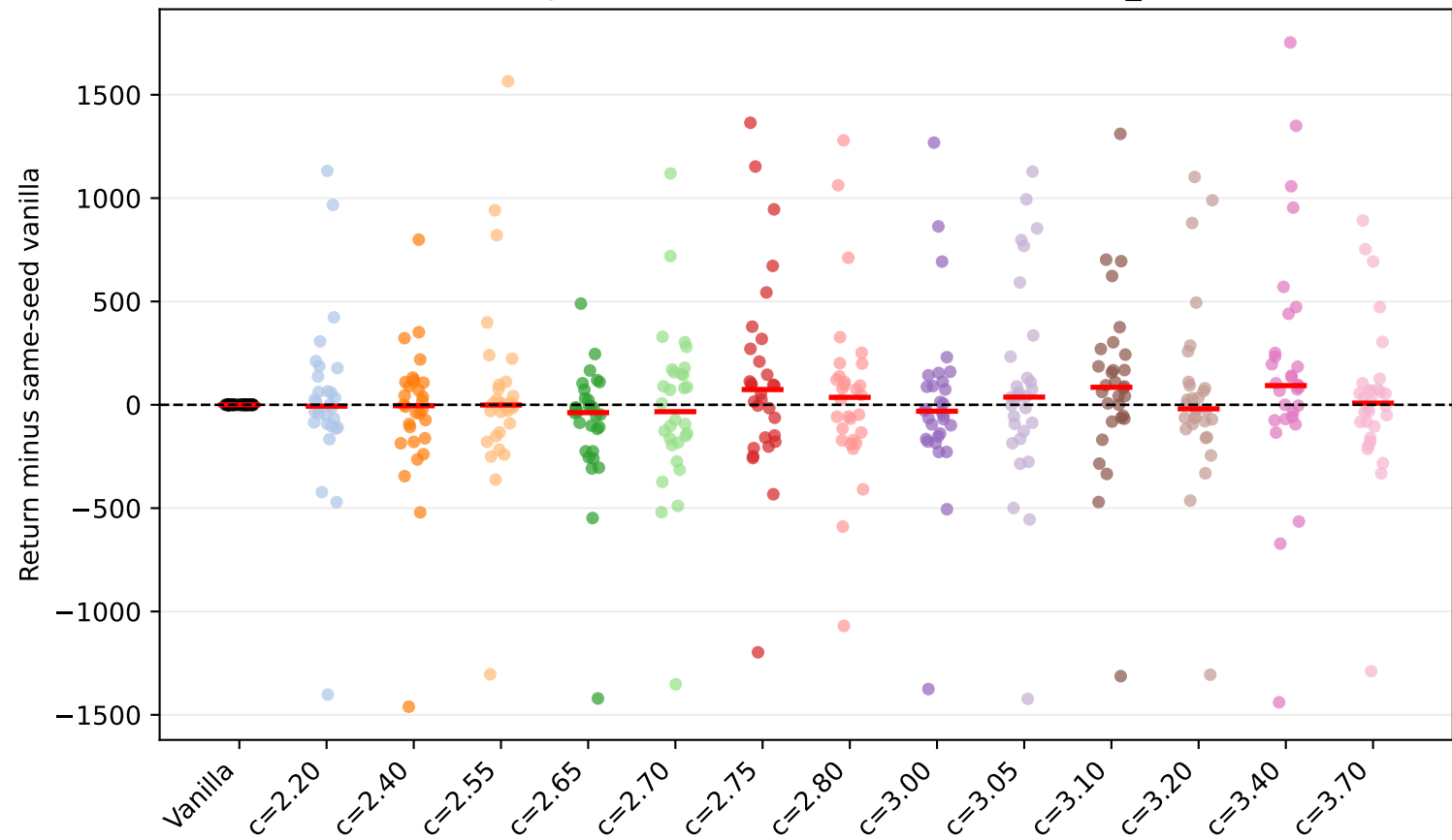
HalfCheetah-v4 gear factor=0.5: seed scatter (vanilla_subtracted)
