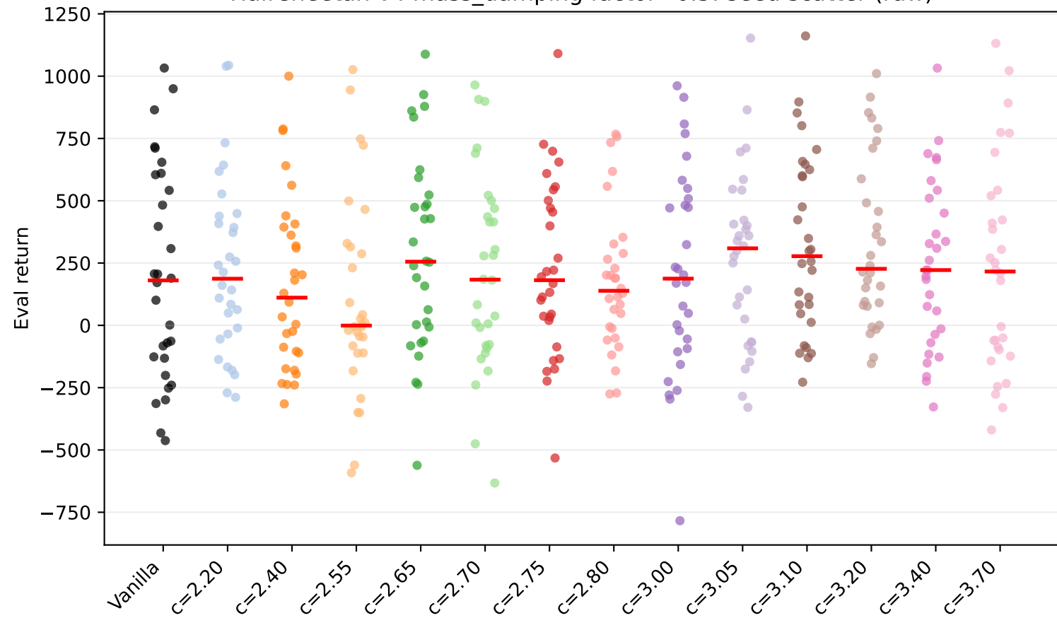
HalfCheetah-v4 mass_damping factor=0.5: seed scatter (raw)
